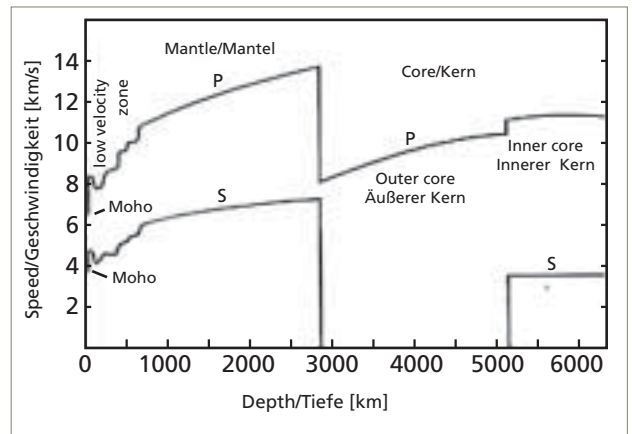
»2 Seismic velocities of P/S-waves, from [1]
